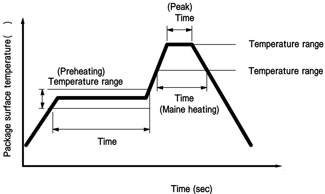
Recommending reflow temperature profile
