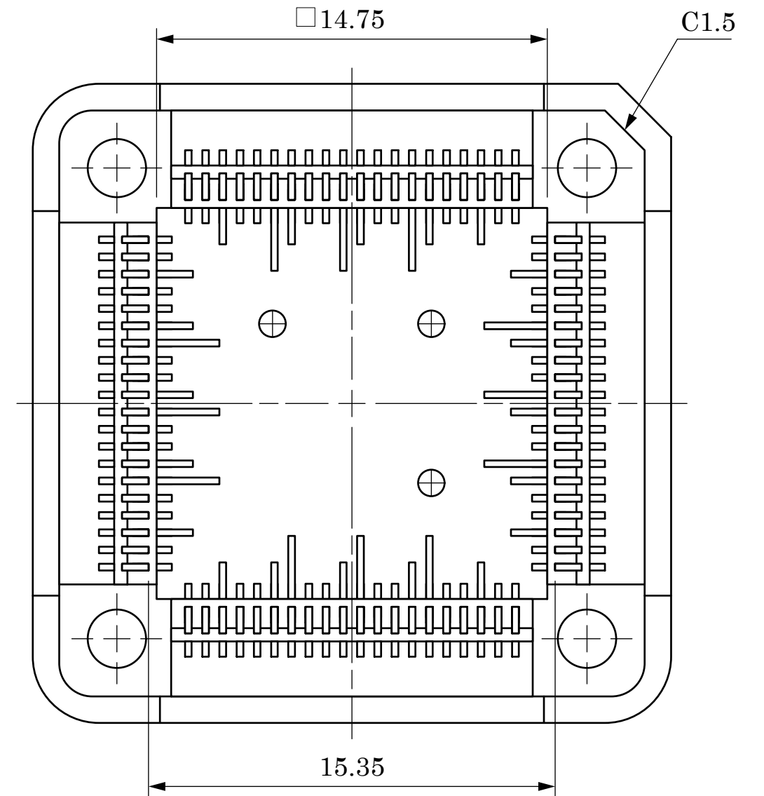
BOTTOM VIEW
