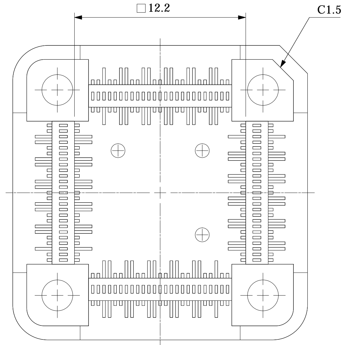
BOTTOM VIEW
