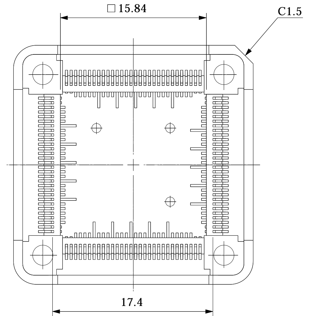
BOTTOM VIEW
