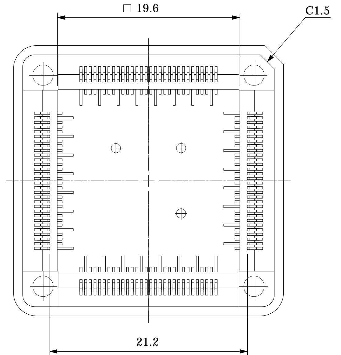
BOTTOM VIEW
