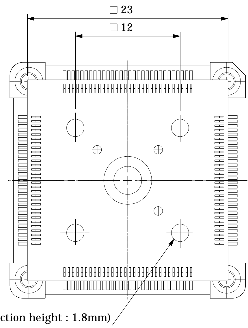
BOTTOM VIEW
