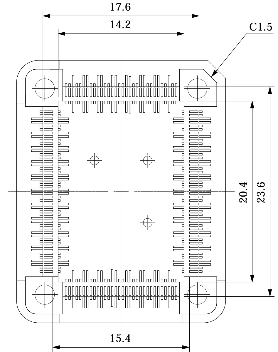
BOTTOM VIEW
