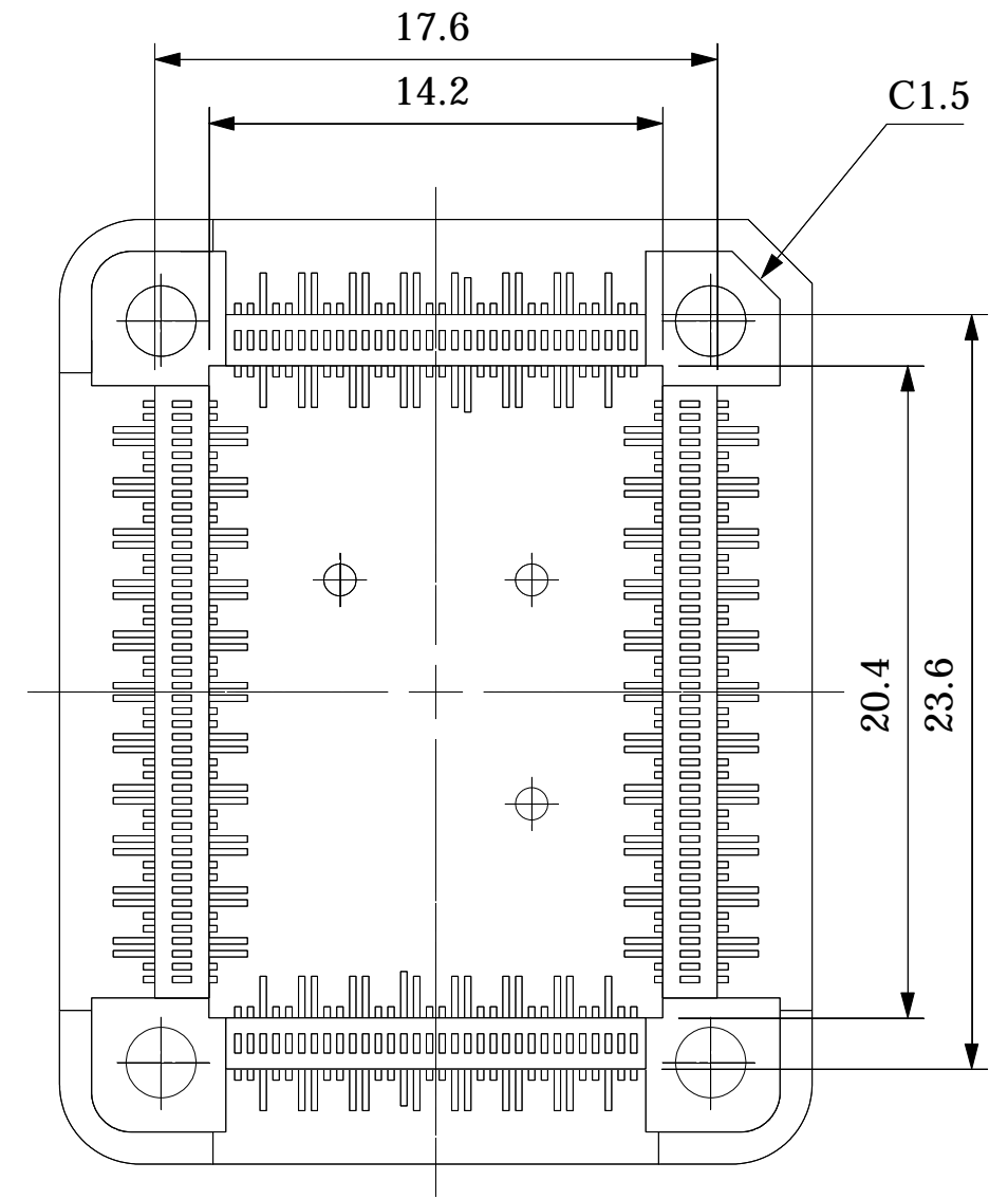
BOTTOM VIEW
