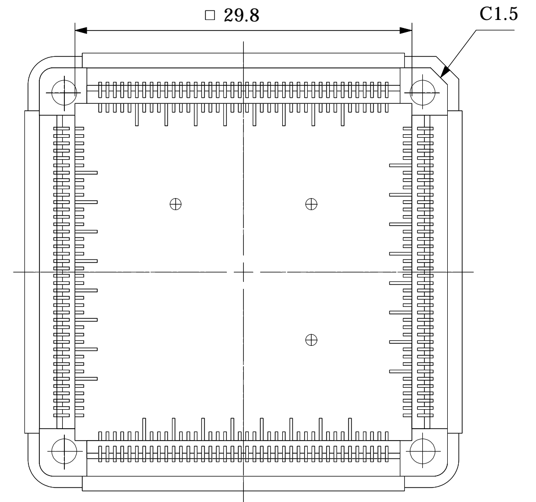
BOTTOM VIEW
