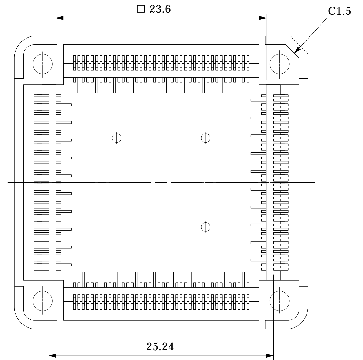
BOTTOM VIEW
