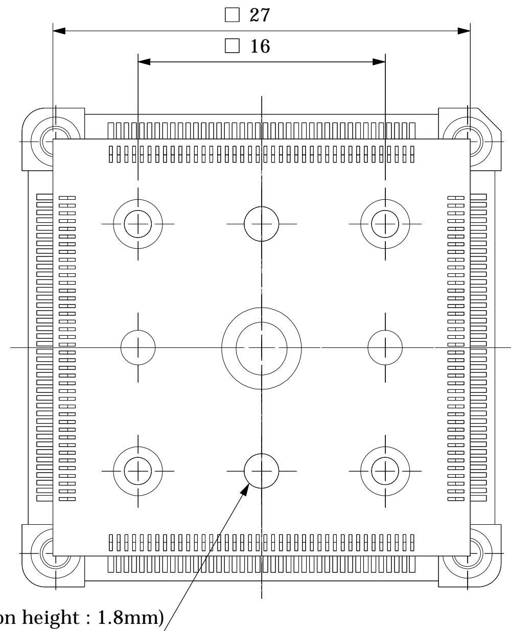
BOTTOM VIEW
