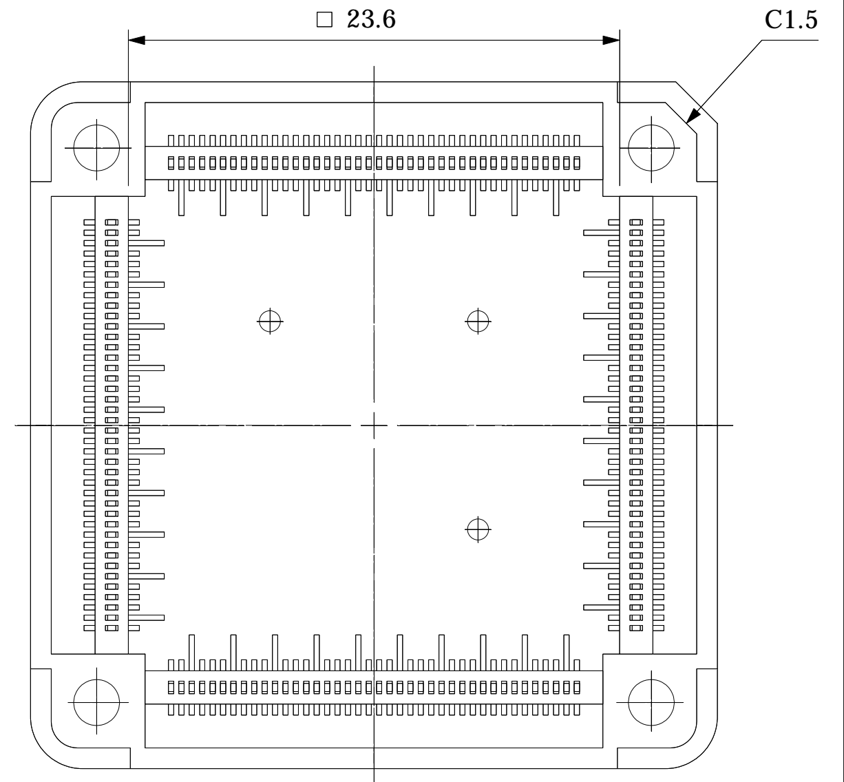
BOTTOM VIEW
