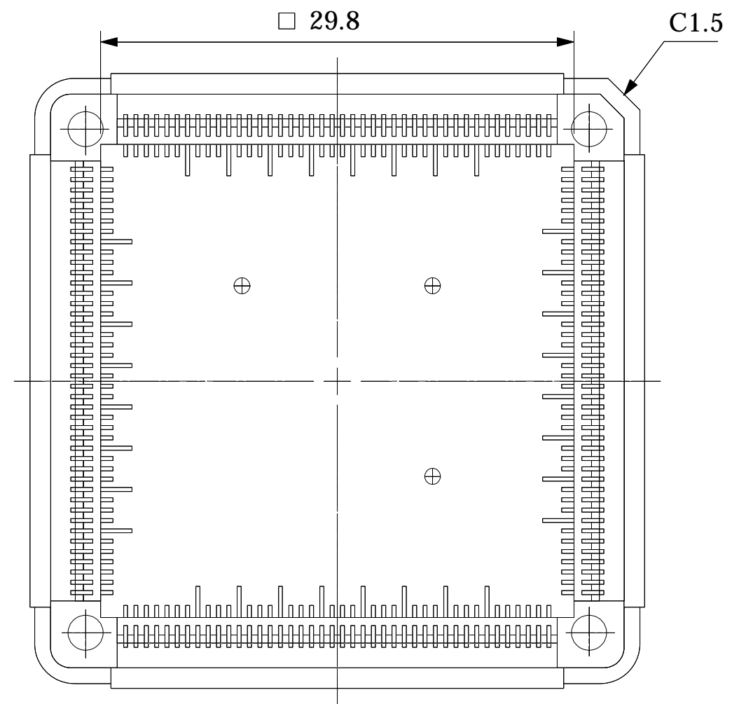
BOTTOM VIEW
