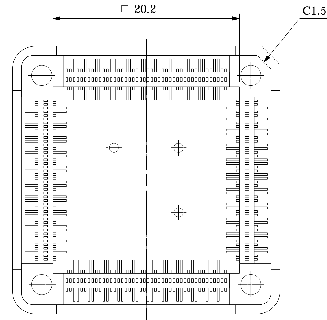
BOTTOM VIEW
