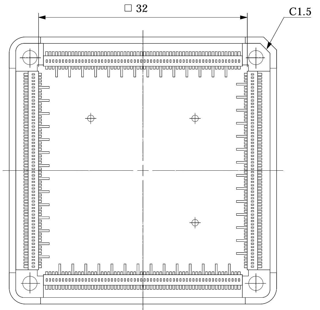
BOTTOM VIEW
