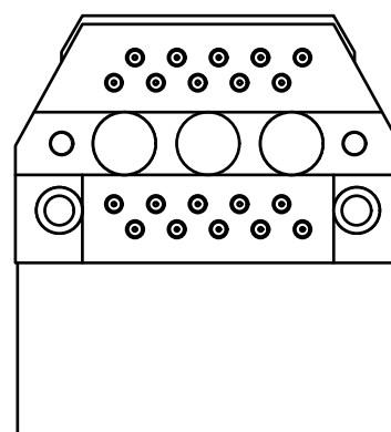
View B
