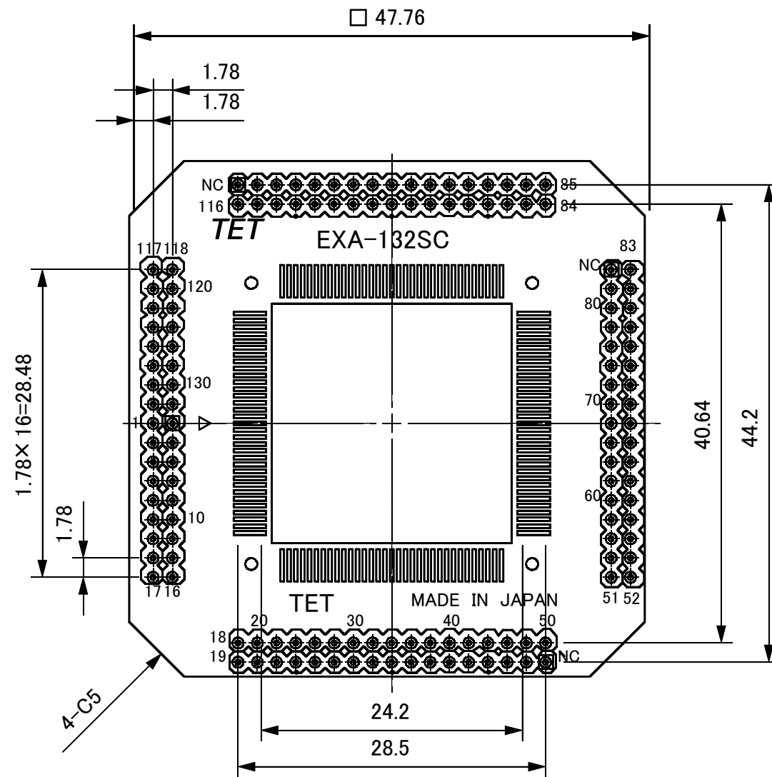
TOP VIEW
