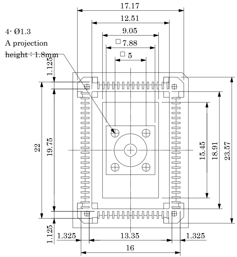
BOTTOM VIEW
