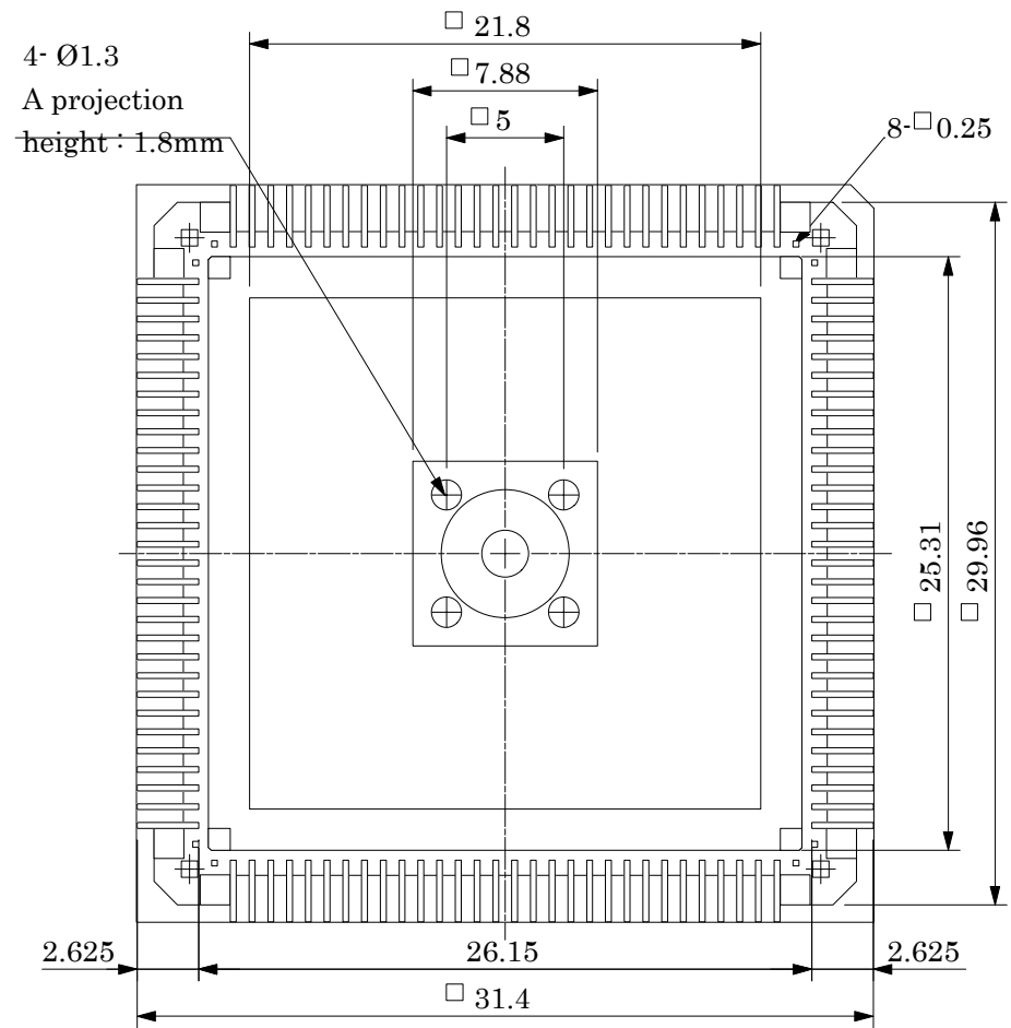
BOTTOM VIEW
