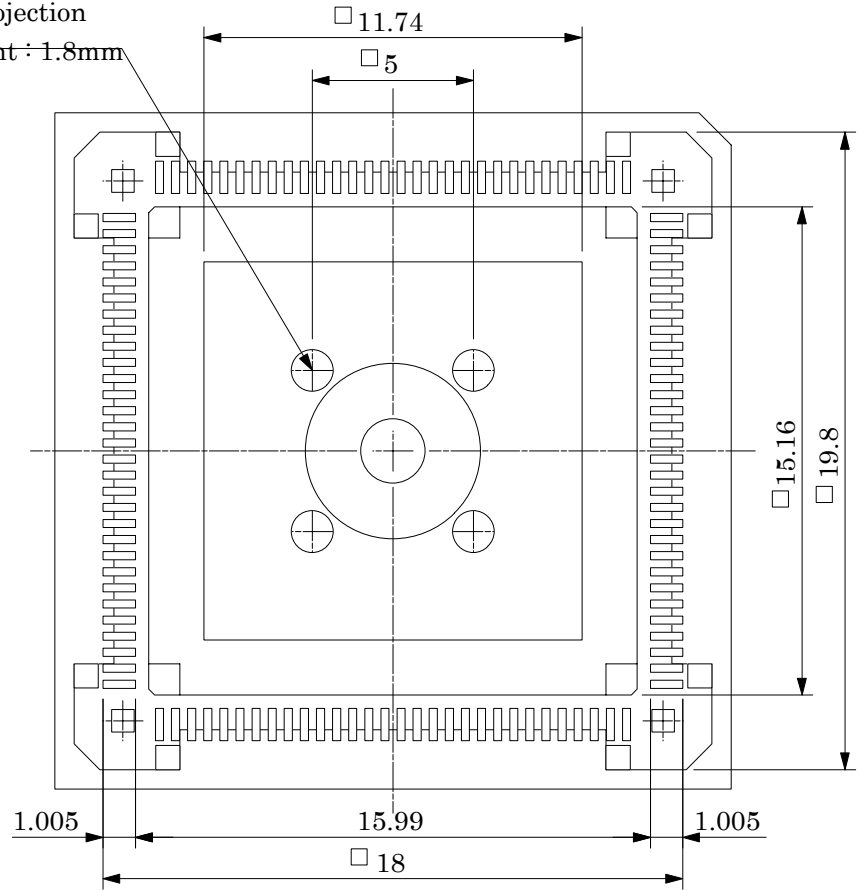
BOTTOM VIEW
