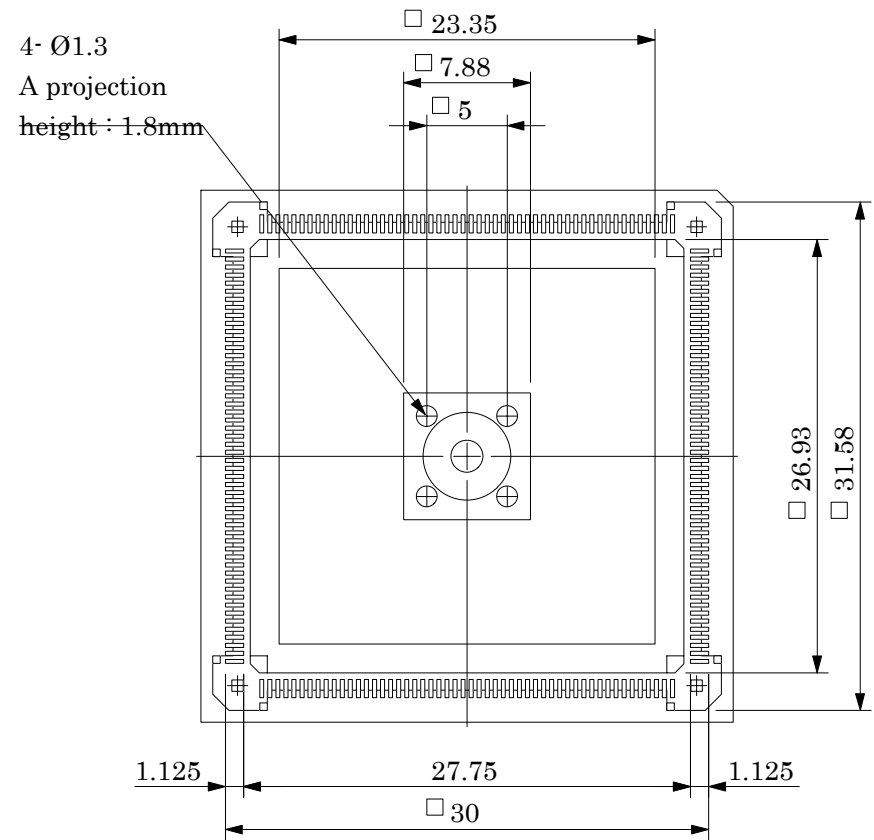
BOTTOM VIEW
